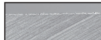
Surface machined with SUMIDIA (Sintered Diamond) wiper insert
